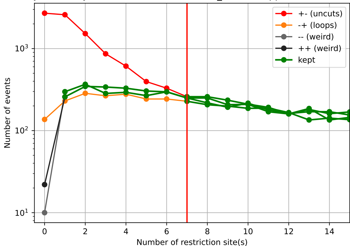
Library events by distance in 1b6c5dedb328_7833^mapped-R64-1-1^WL4
